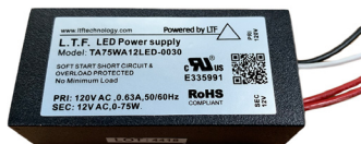
60W & 75W 12V Electronic Transformer (60WLEDTRANS, 75WLEDTRANS) 60 & 75 Watt 12V Electronic Transformer
